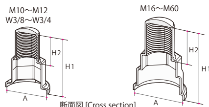
断面図 [Cross section]
