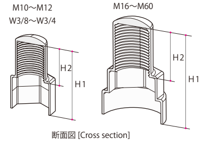
断面図 [Cross section]
