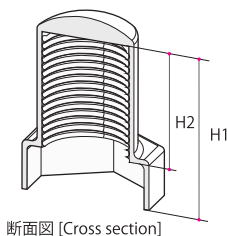
断面図 [Cross section]
